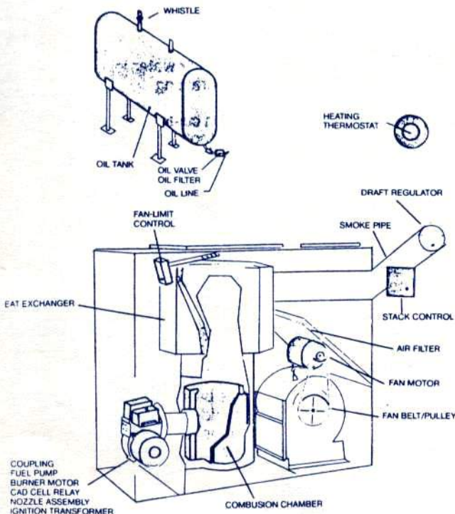
WARM AIR HEATER
