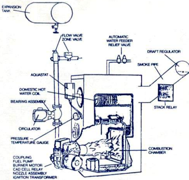
HOT WATER BOILER
